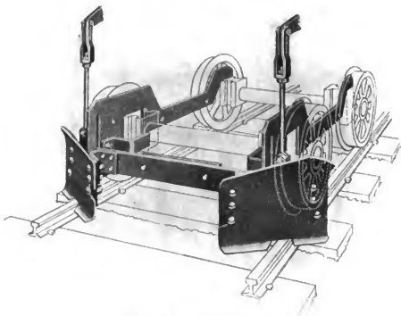
Fig. 2408. Priest Snow Flanger. Quincy, Manchester, Sargent Co.
